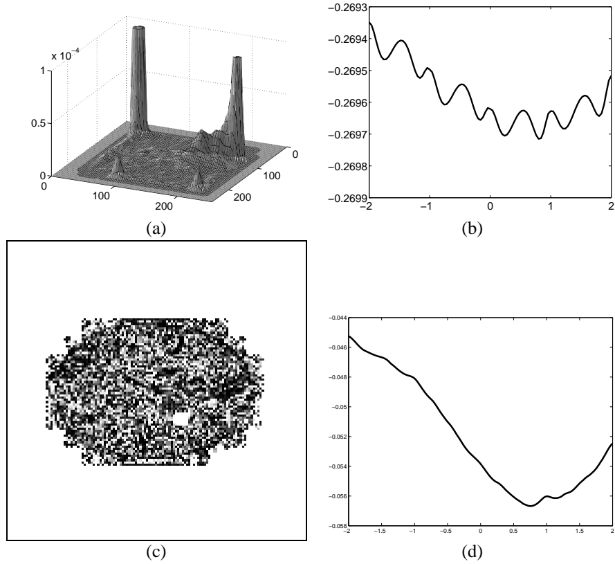
Fig. 2. Distance measures versus shifts; (a) the joint density approximation for R and T , (b) mutual information versus shift, (c) the normalized gradient field for R and T , (d) normalized gradient field versus shift.
