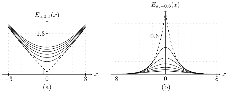
FIG. 1. The dashed lines in both figures denote the graph of e^{\beta|x|} . The solid lines from bottom to top are E_{a,\beta}(x) with the parameter a ranging from 1 to 6 for Figure 1(a) and from 6 to 1 for Figure 1(b), which are representative of the cases \beta > 0 and \beta < 0 , respectively. The parameter \beta controls the asymptotic behavior near infinity while both a and \beta determine how the function e^{\beta|x|} is smoothed at zero. The smaller a is, the closer E_{a,\beta}(0) is to 1.
